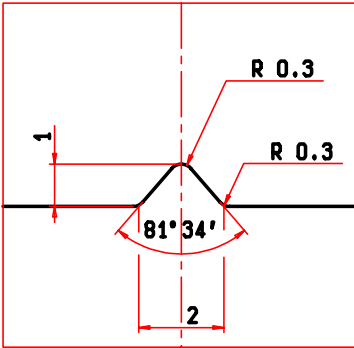
PART. "U" SCALA 8:1
